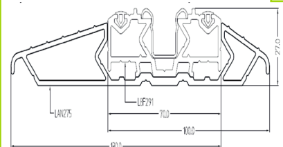
LOW ALUMINIUM THRESHOLD WITH RAMP
