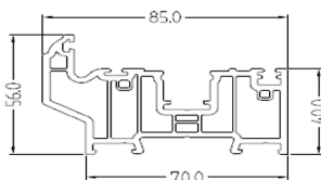
LBF091 Outer Frame PVC THRESHOLD
