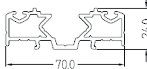
LBF291 Low Threshold LOW ALUMINIUM THRESHOLD
